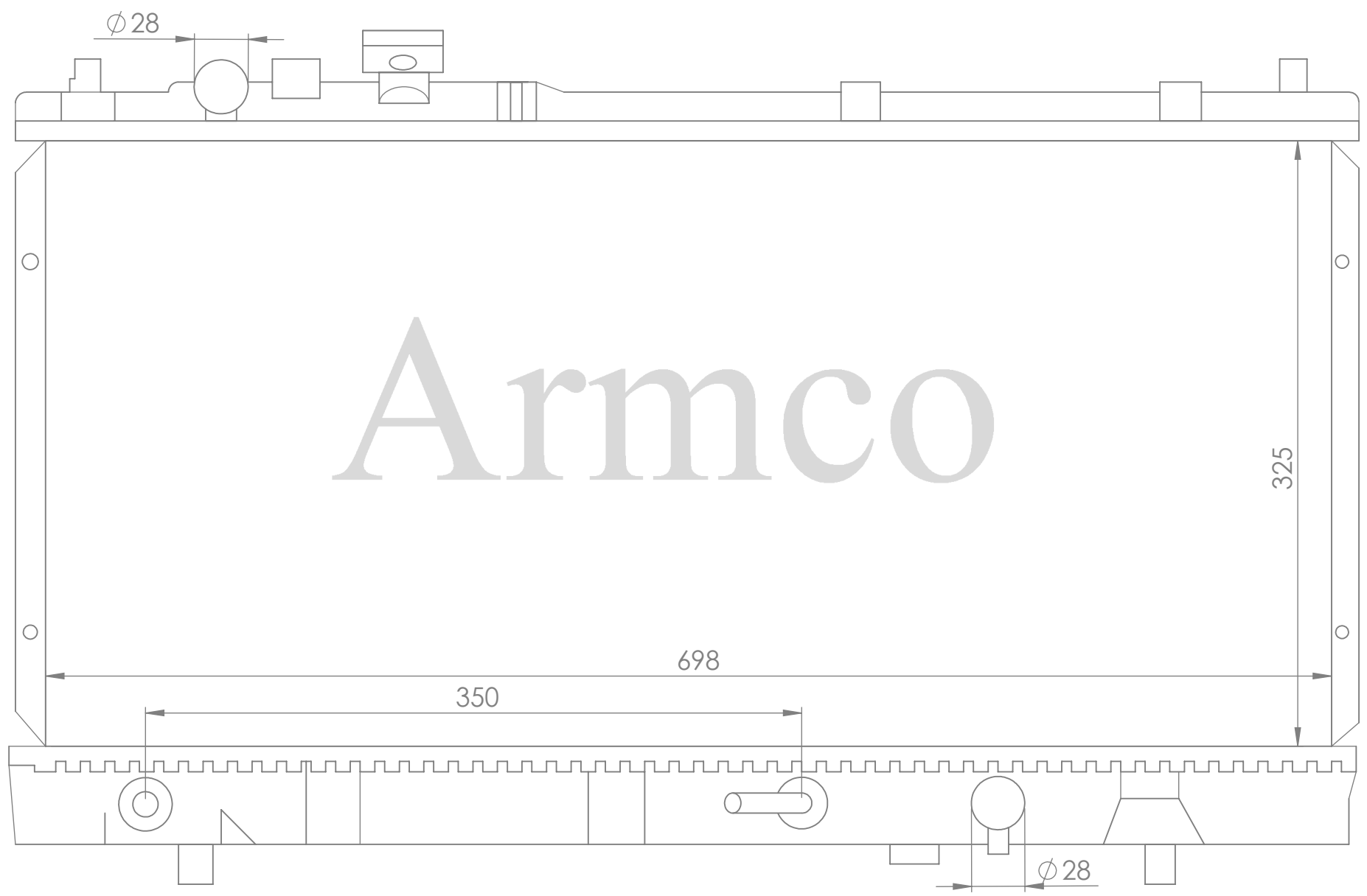
Core Size:325x698x16/26
